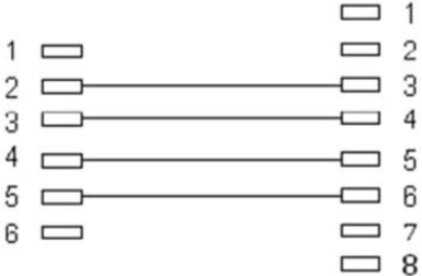
RJ11/14 (6P4C)
