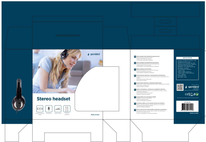
size: 190x74x188 mm
